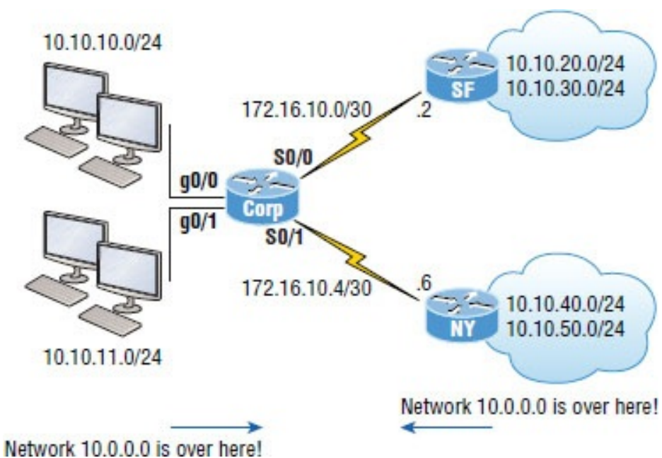
FIGURE 17.6 Discontiguous networks
