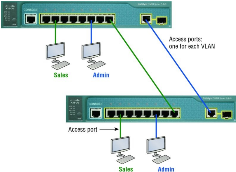
FIGURE 11.5 Access ports
