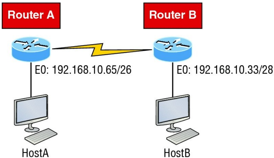
FIGURE 5.19 Find the valid host #2
