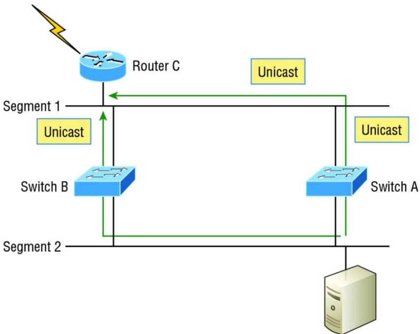
FIGURE 10.8 Multiple frame copies
