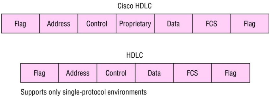
FIGURE 21.10 Cisco's HDLC frame format: Each vendor's HDLC has a proprietary data field to support multiprotocol environments. The reason every vendor has a
