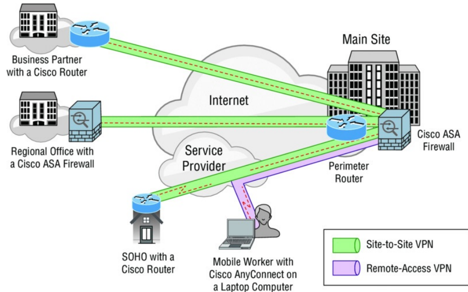
FIGURE 21.21 Enterprise-managed VPNs
