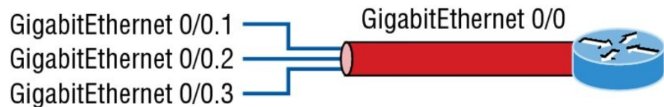
FIGURE 11.10 A router creates logical interfaces.
