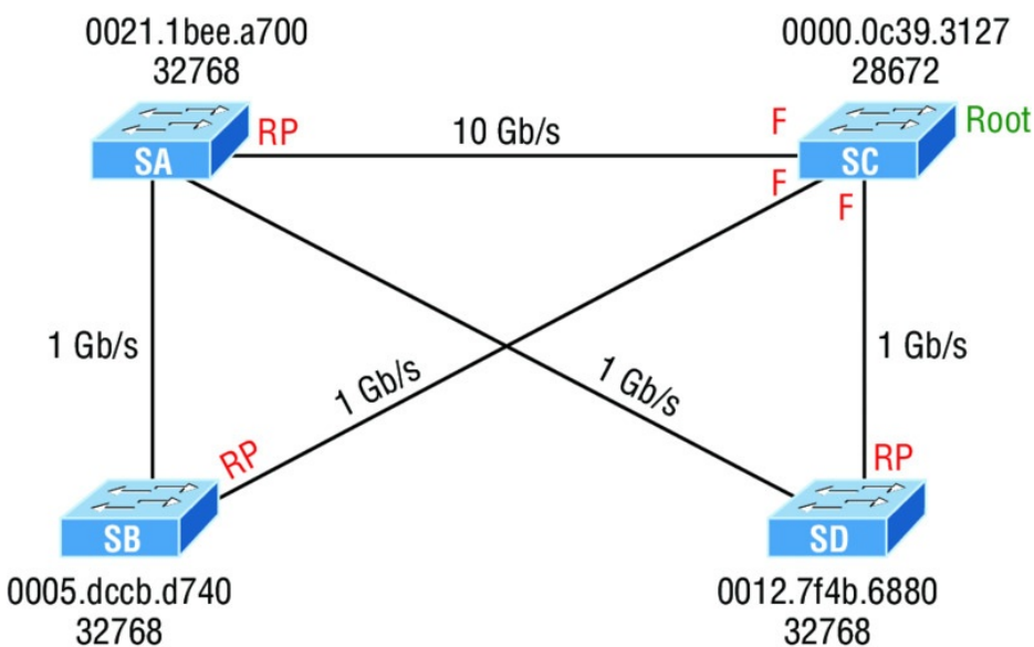
FIGURE 15.14 RSTP example 2, answer 1
