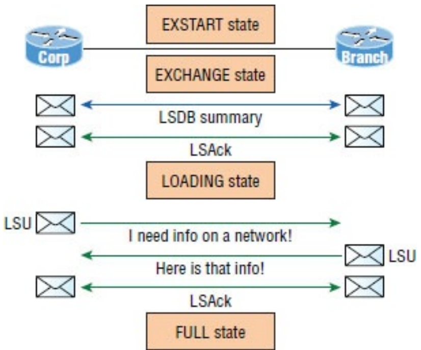
Figure 19.7 OSPF router neighbor states, part 2
