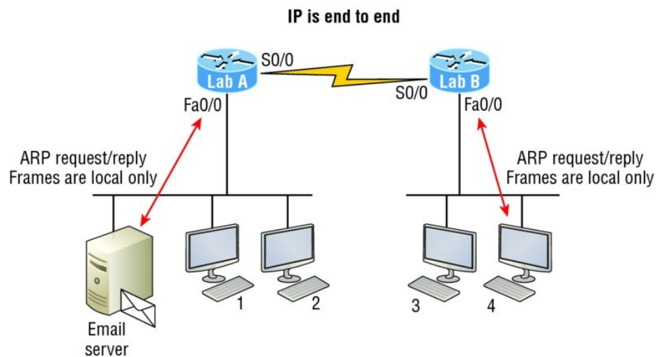
FIGURE 9.7 Testing basic routing knowledge
