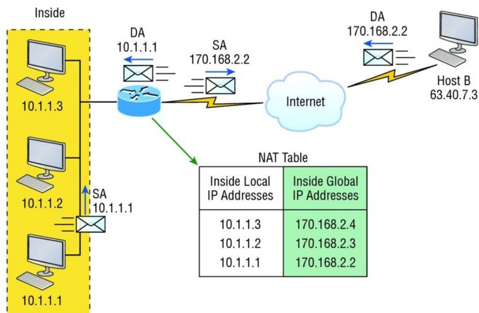
FIGURE 13.2 Basic NAT translation
