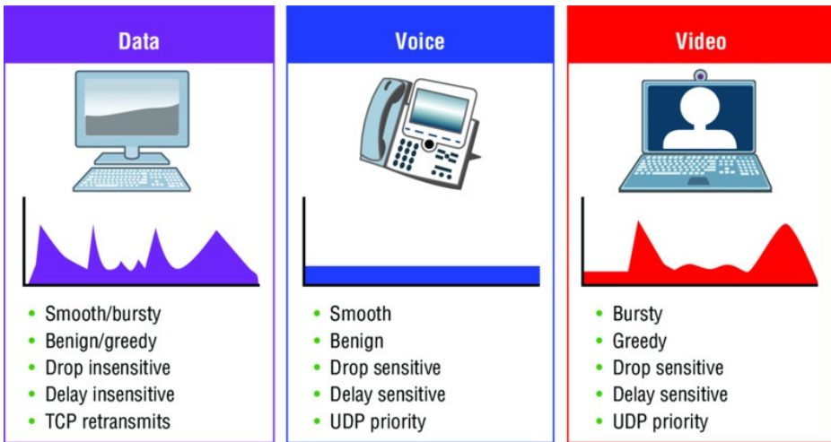
FIGURE 22.12 Traffic characteristics
