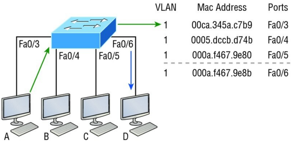
FIGURE 10.4 Forward/filter table answer
