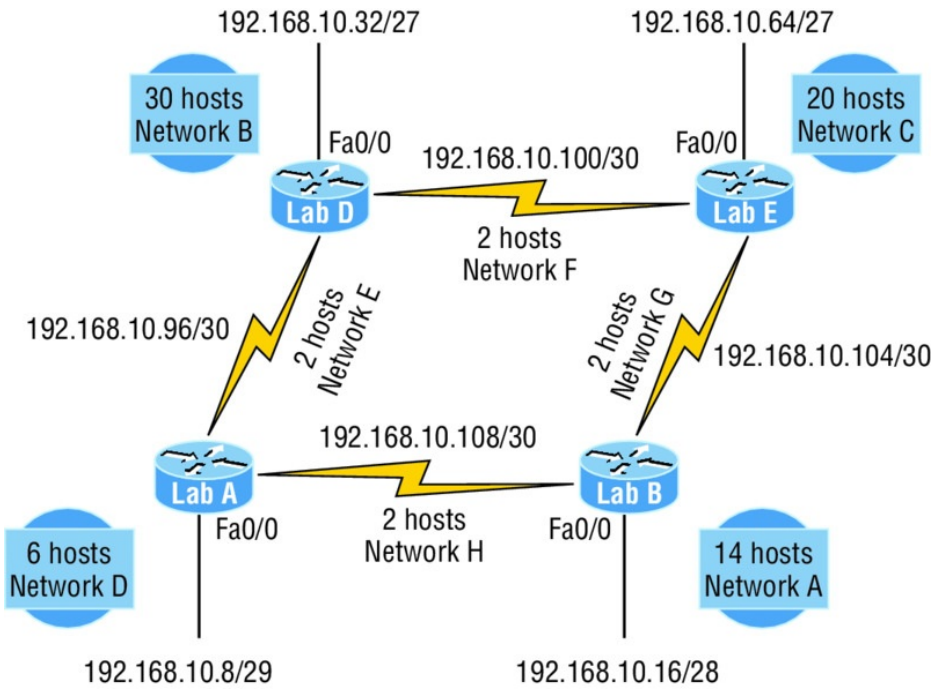
FIGURE 5.4 VLSM network example
