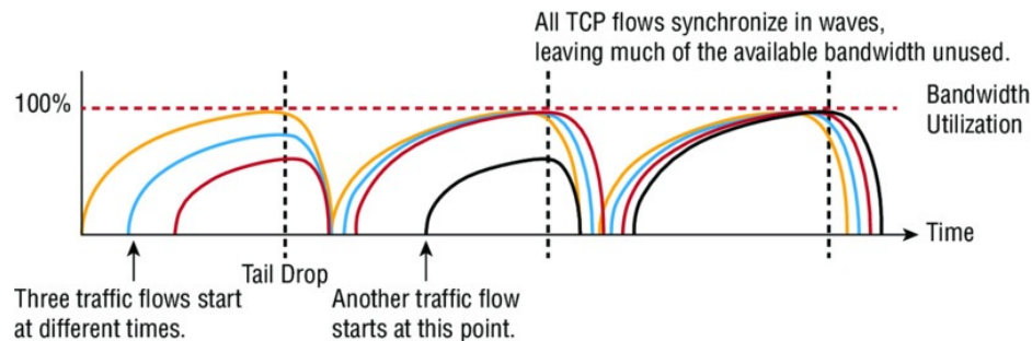
FIGURE 22.17 Congestion avoidance
