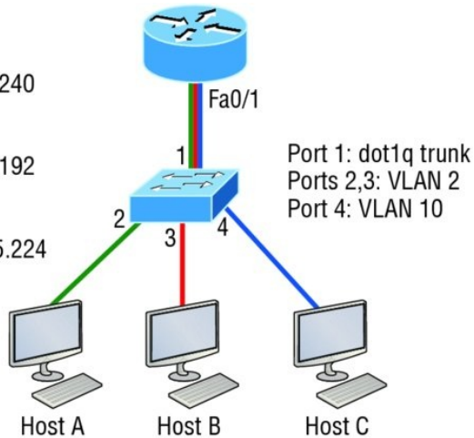
FIGURE 11.12 Configuring inter-VLAN example 1
