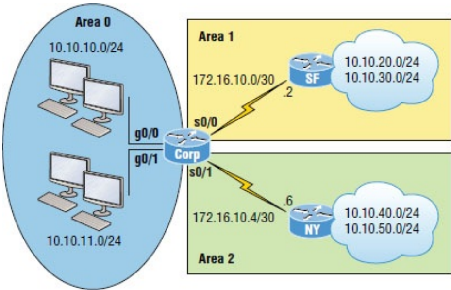
Figure 19.8 Our internetwork
