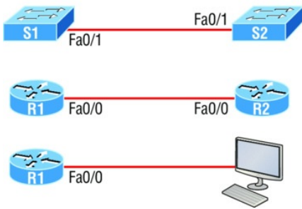
FIGURE 2.12 Typical uses for straight-through and cross-over Ethernet cables
