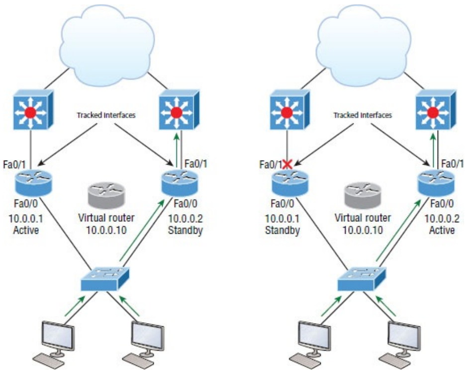
Figure 16.12 Interface tracking setup
