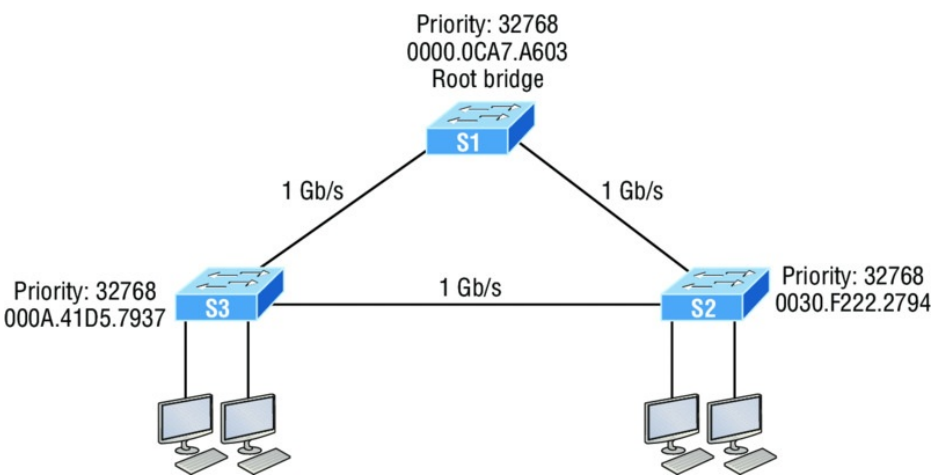
FIGURE 15.4 STP operations
