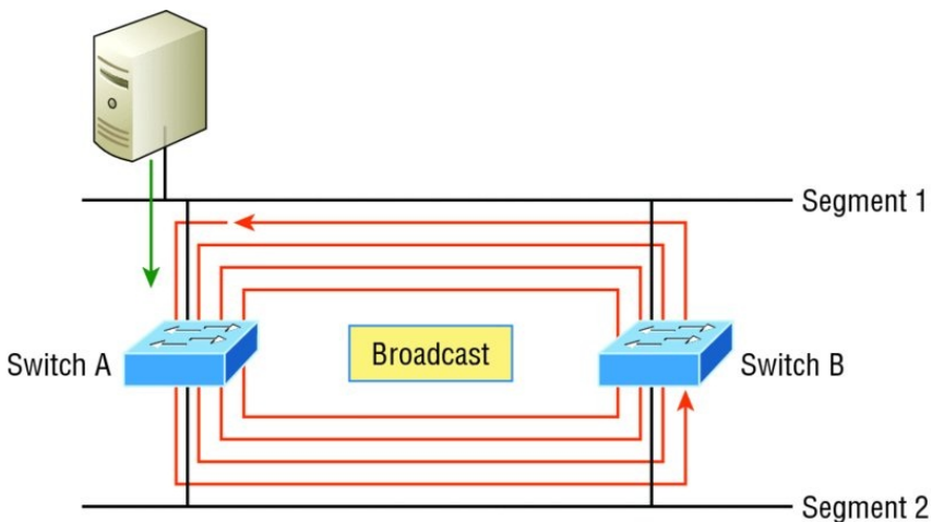
FIGURE 10.7 Broadcast storm
