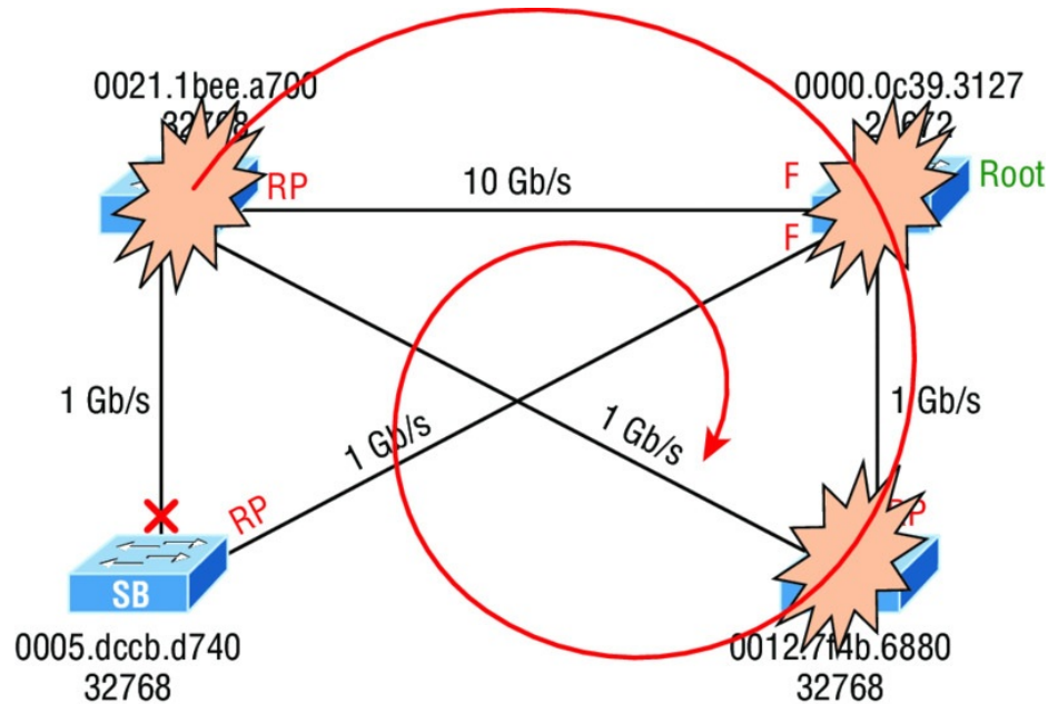
FIGURE 15.18 STP failure
