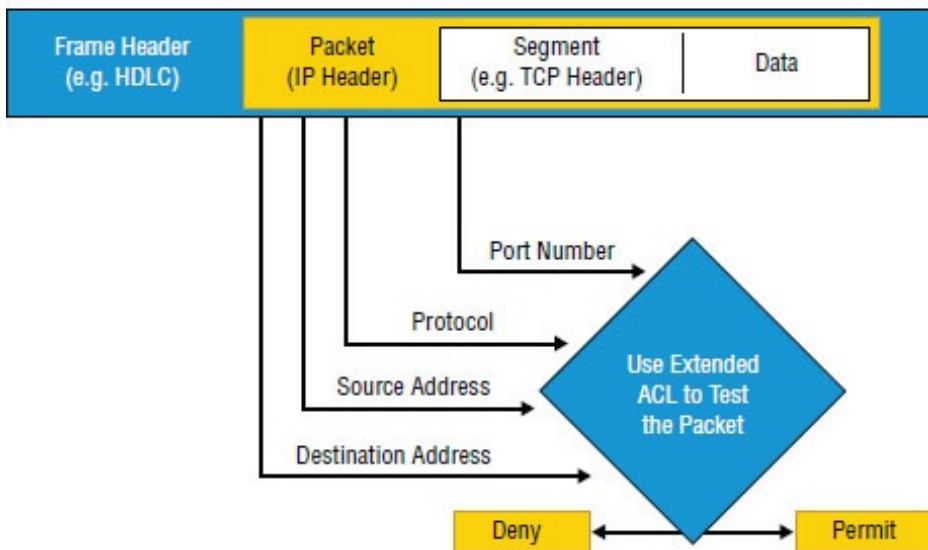
Figure 20.3 Extended ACLs
