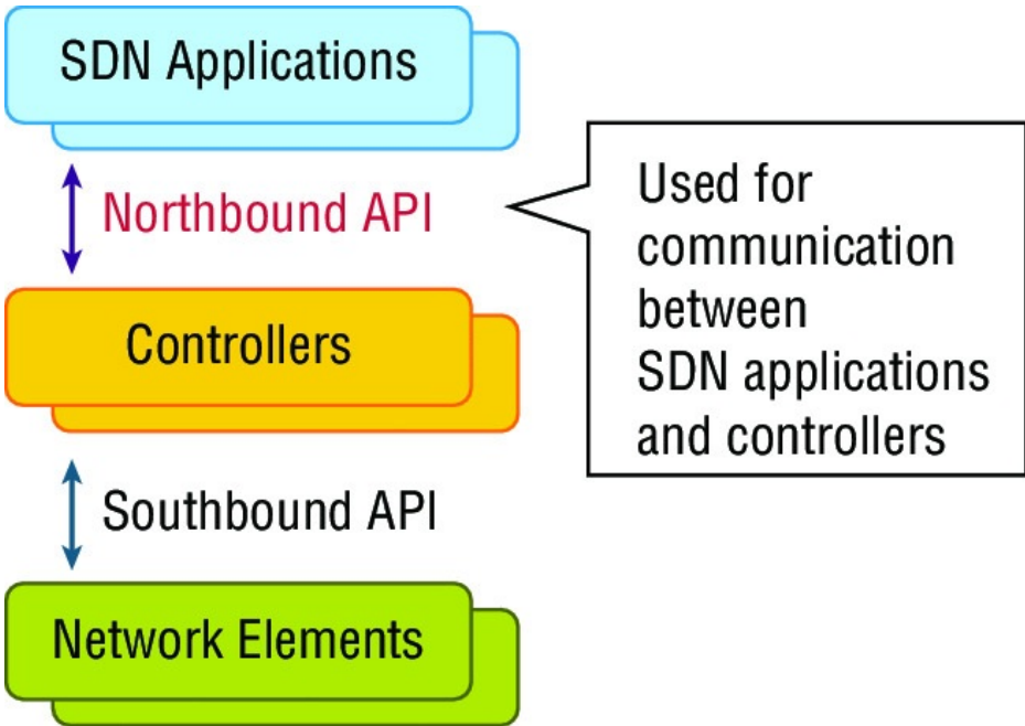
FIGURE 22.7 Northbound interfaces
