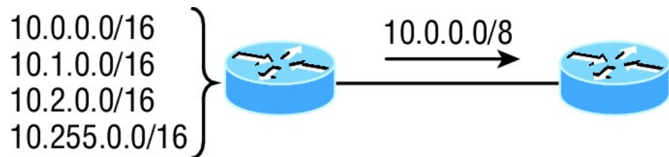
FIGURE 5.12 Summary address used in an internetwork
