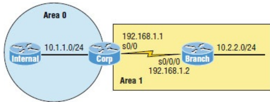
Figure 19.9 Our internetwork
