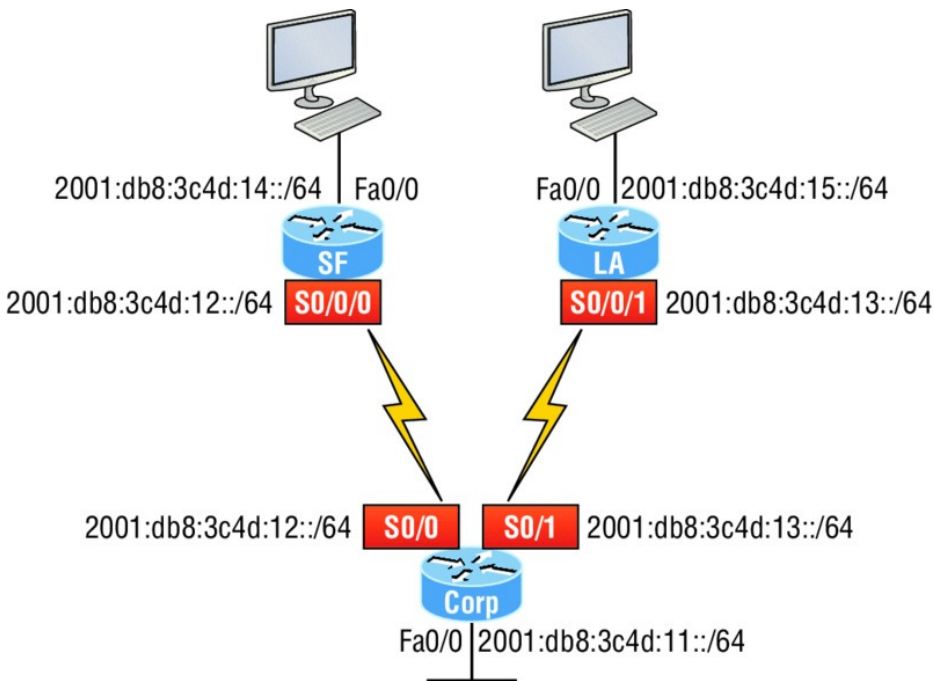
FIGURE 14.13 Our internetwork
