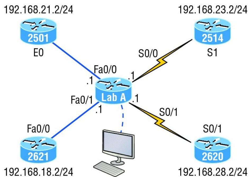
FIGURE 7.8 Network topology documented
