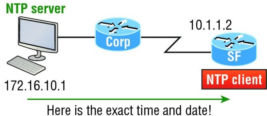
FIGURE 7.5 Synchronizing time
