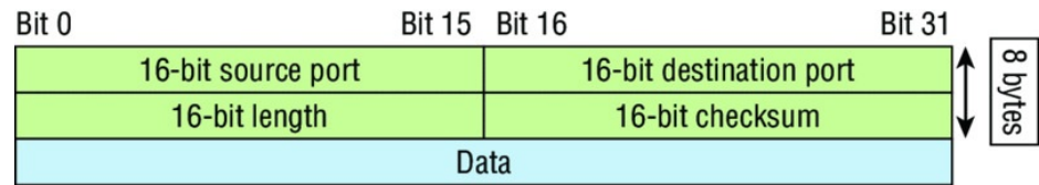
FIGURE 3.13 UDP segment
