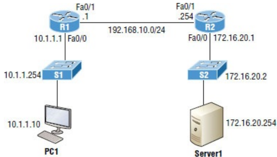
Figure 20.1 Troubleshooting scenario
