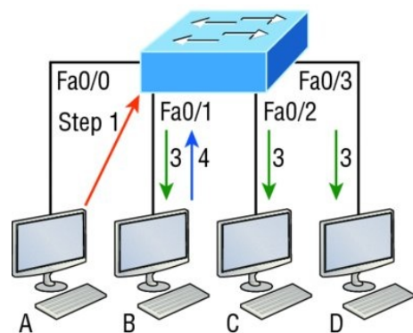
CAM/MAC forward/filter table
