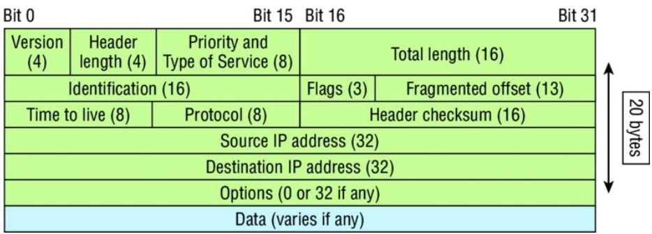
FIGURE 3.15 IP header
