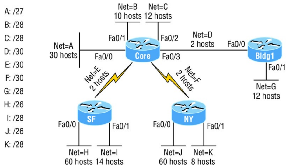
FIGURE 5.6 VLSM network example
