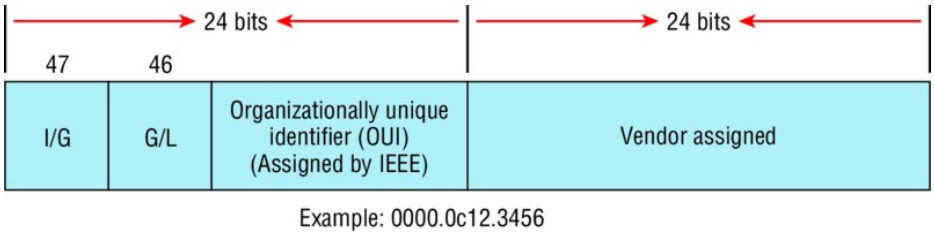
FIGURE 2.7 Ethernet addressing using MAC addresses
