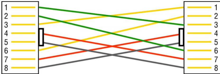
FIGURE 2.13 UTP Gigabit crossover Ethernet cable
