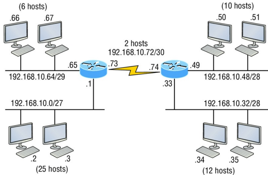
FIGURE 5.2 Classless network design
