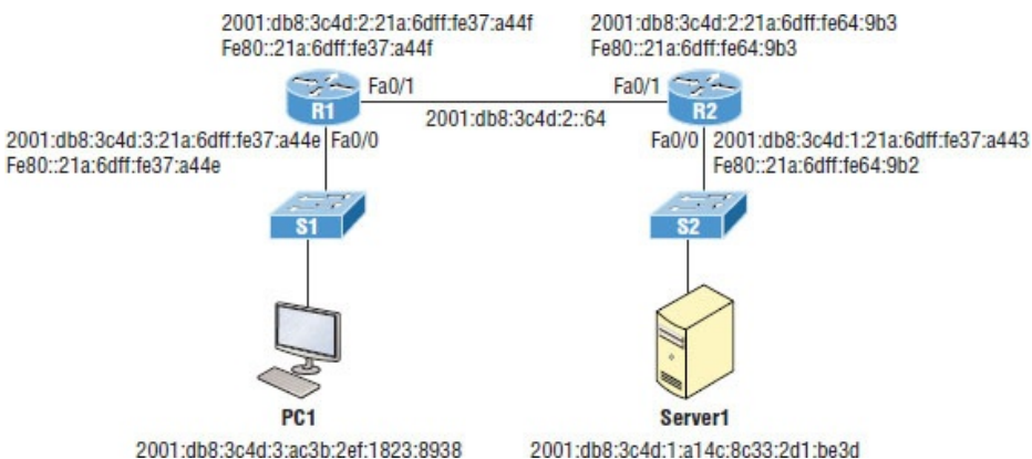
Figure 20.4 IPv6 troubleshooting scenario
