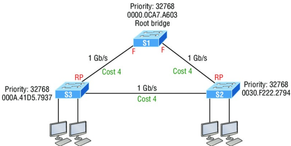
FIGURE 15.5 STP operations
