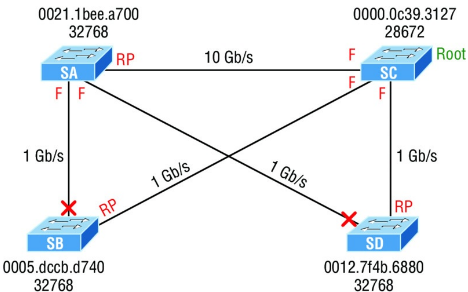
FIGURE 15.17 STP stopping loops
