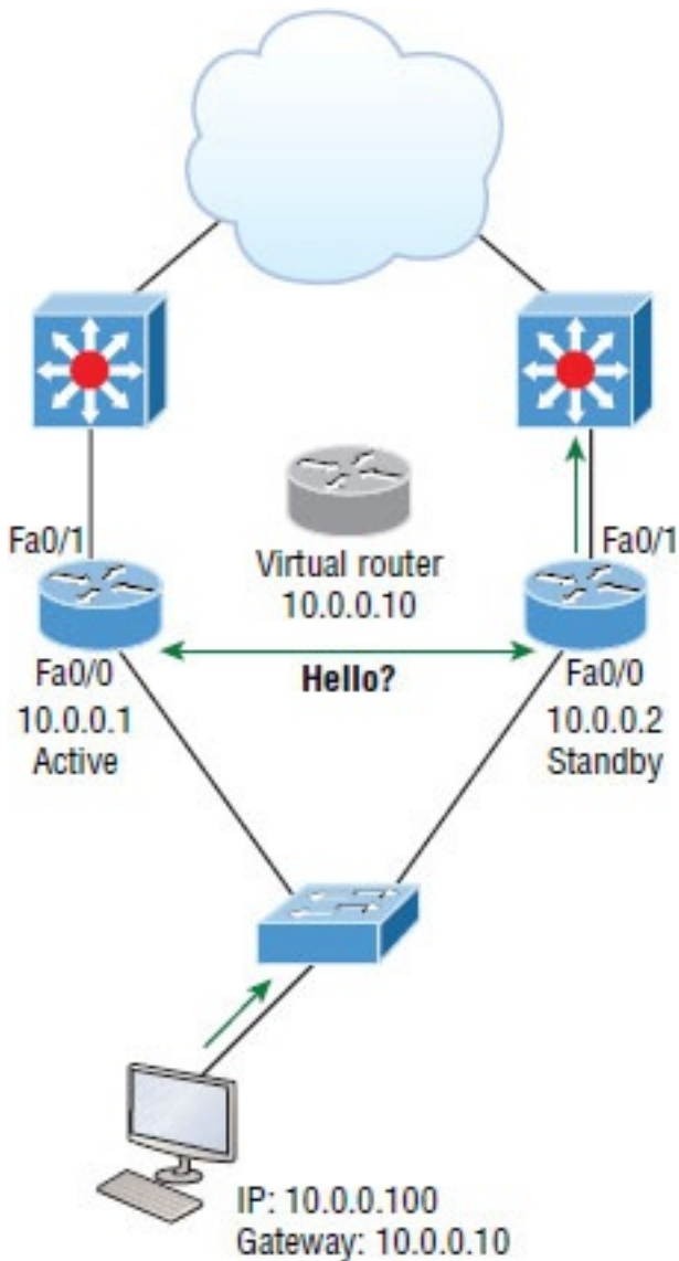
Figure 16.11 HSRP Hellos
