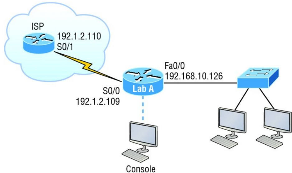
FIGURE 13.5 Another NAT example
