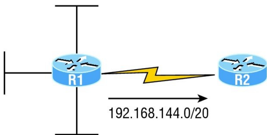
FIGURE 5.13 Summarization example 4
