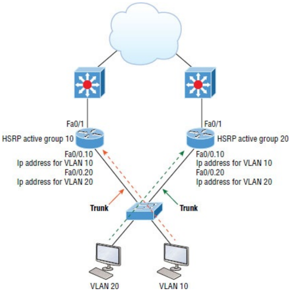
Figure 16.14 HSRP load balancing per VLAN
