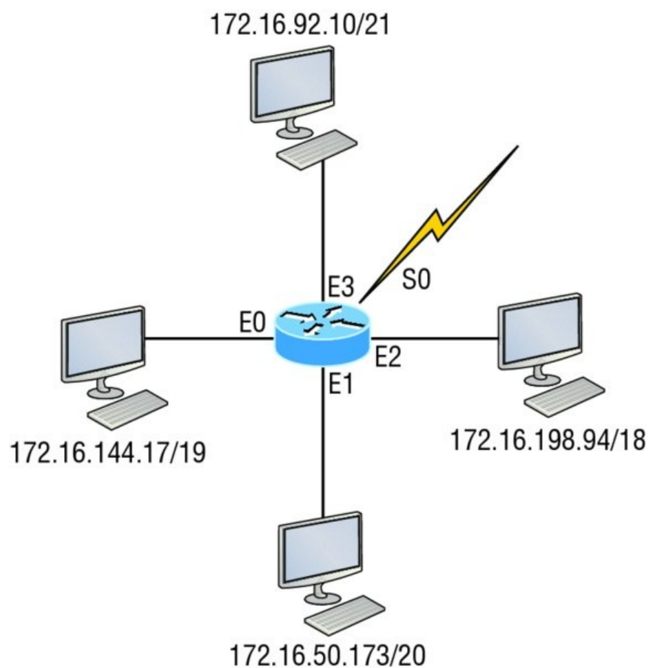
FIGURE 12.4 IP standard access list example 3
