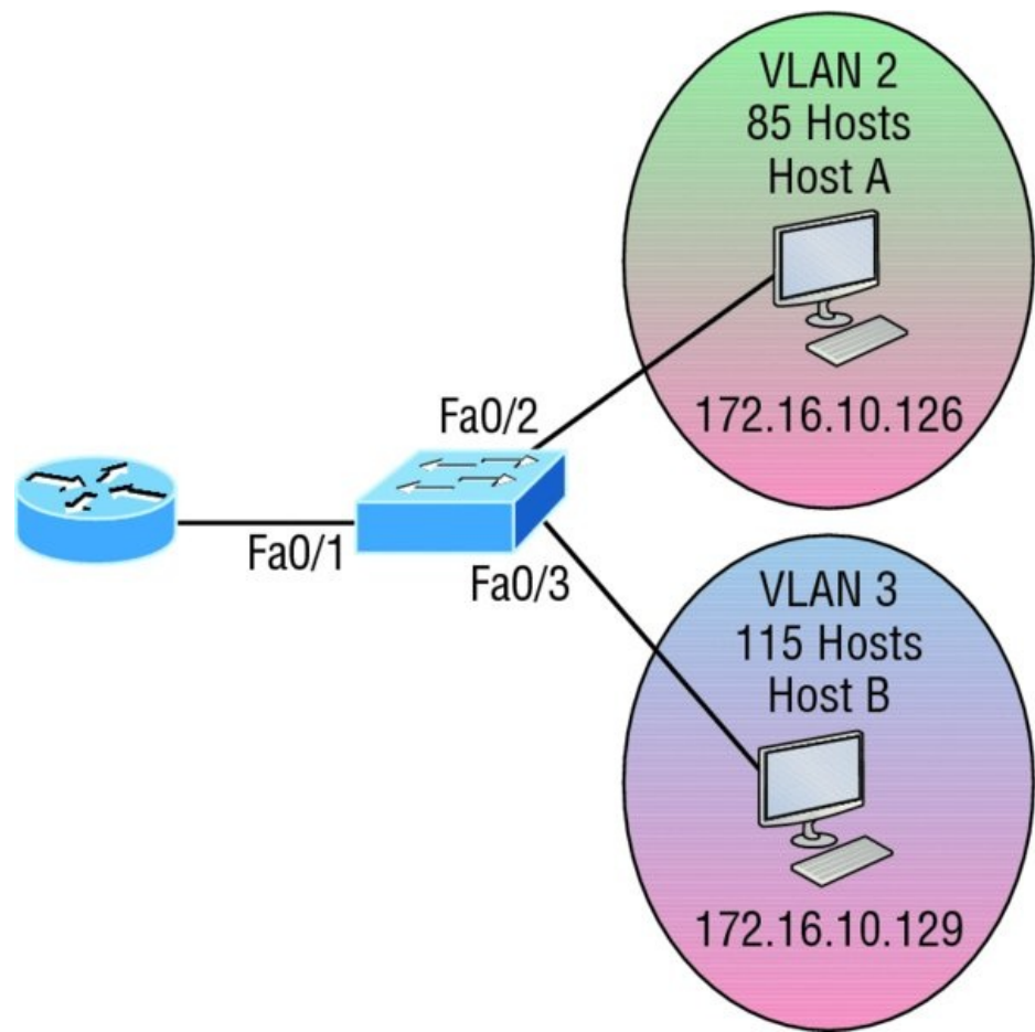
FIGURE 11.14 Inter-VLAN example 3
