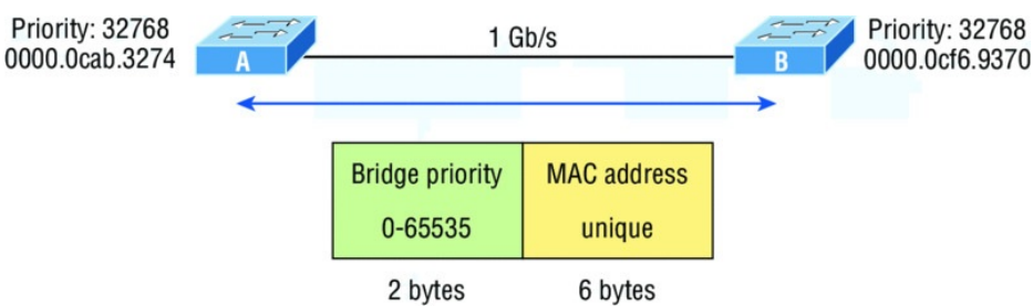
FIGURE 15.7 STP operations
