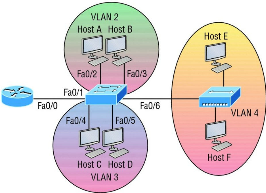
FIGURE 11.13 Inter-VLAN example 2
