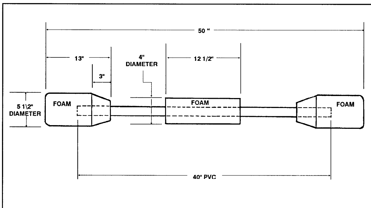
Figure A-6. Materials in pugil stick construction.
